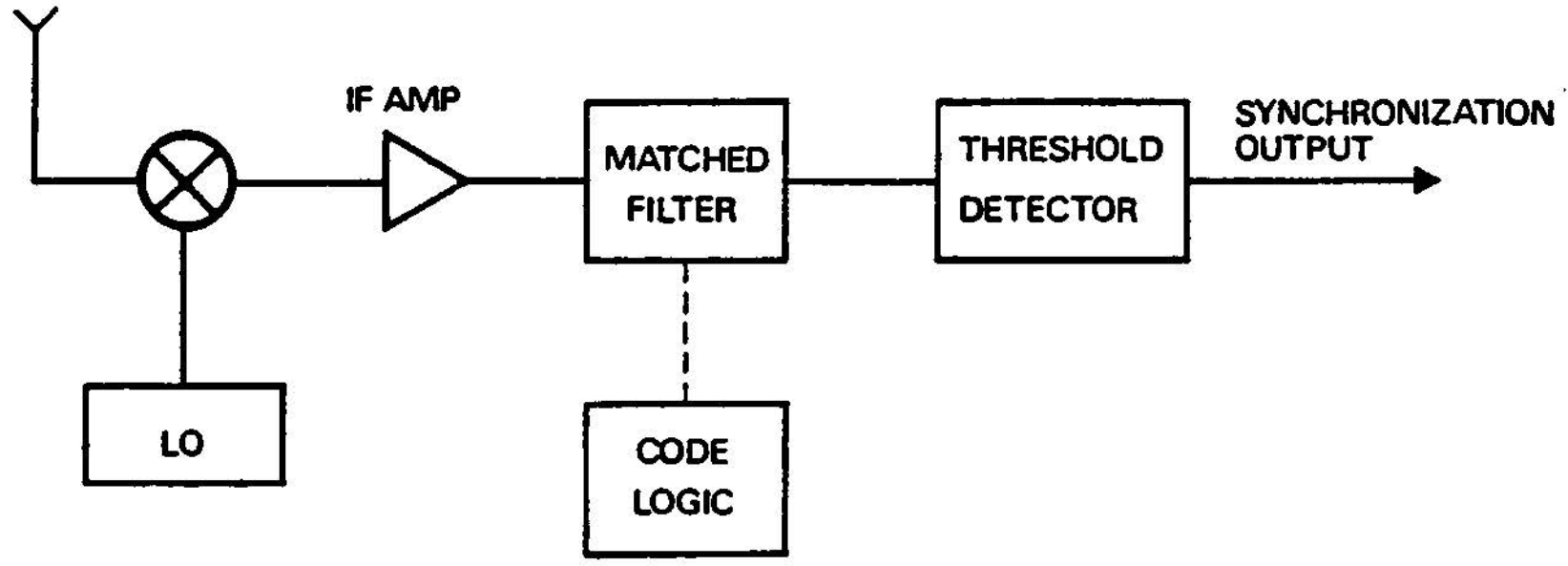
Receiver Synchronization Block
